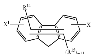
[Chemical Formula 40]
