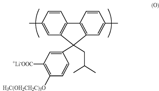
[Chemical Formula 80]
