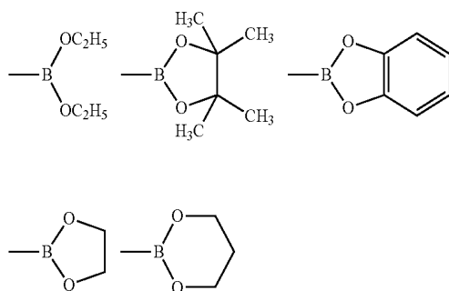
[Chemical Formula 46]
