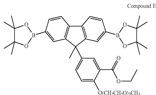
Compound E
