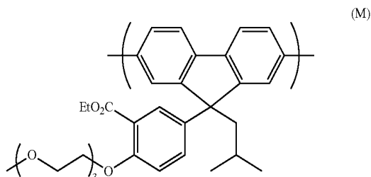
[Chemical Formula 78]
