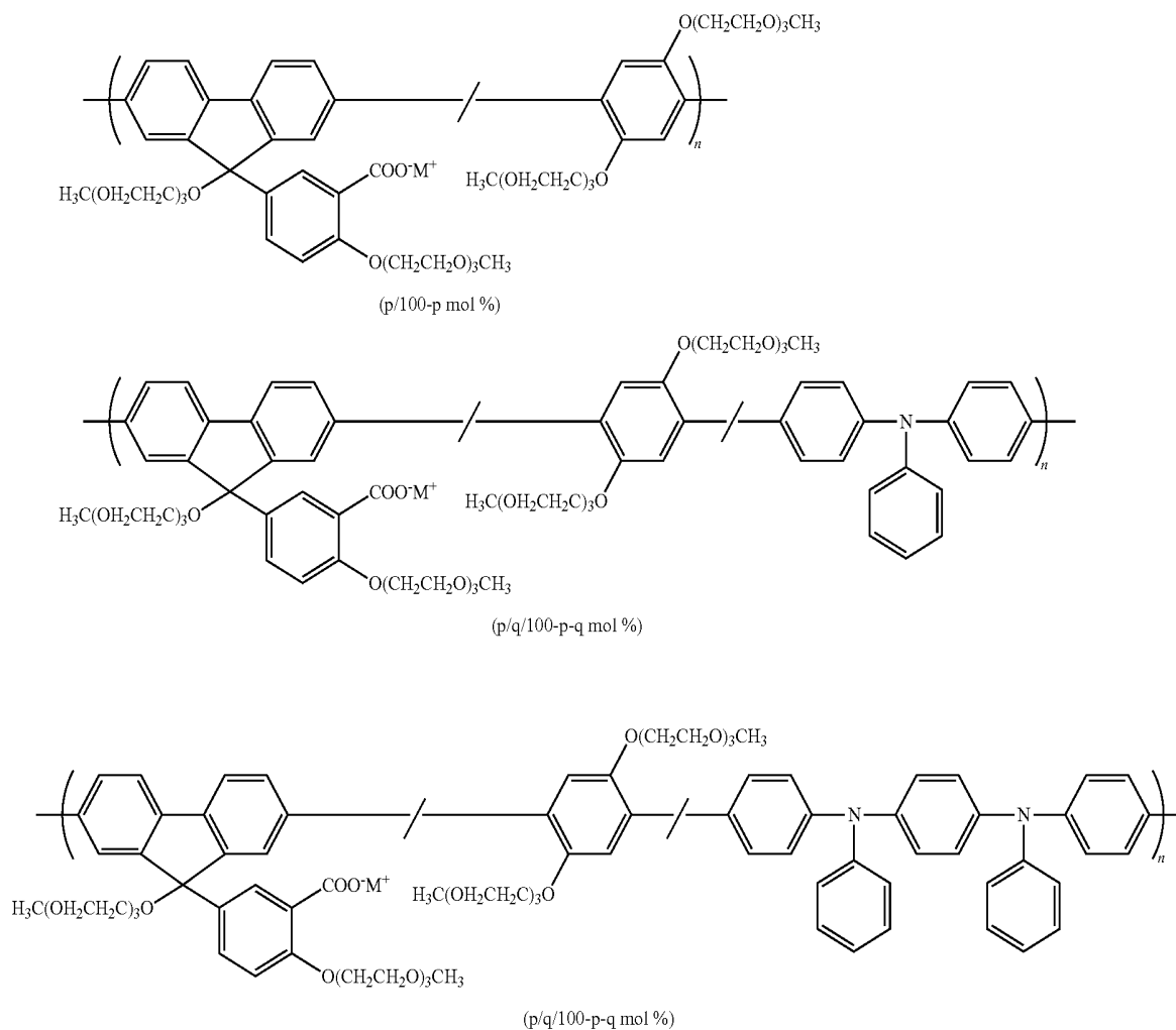
[Chemical Formula 35]
