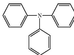
[Chemical Formula 27]
