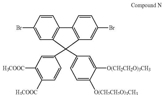
[Chemical Formula 83]
