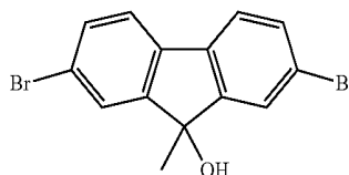
[Chemical Formula 53]
