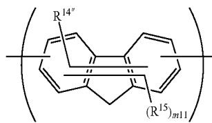
[Chemical Formula 50]
