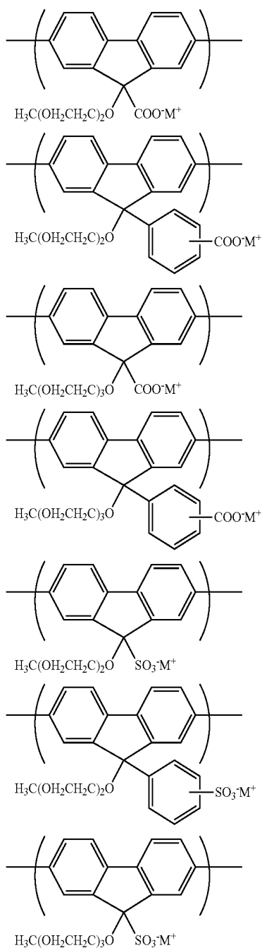
[Chemical Formula 16]
