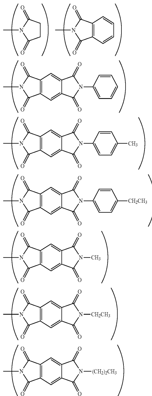
[Chemical Formula 7]
