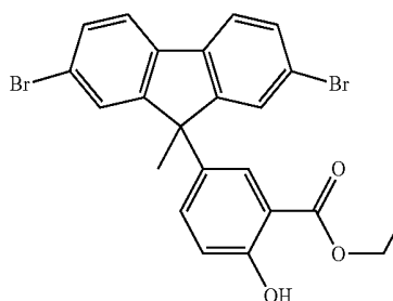
[Chemical Formula 55]
