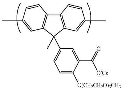
[Chemical Formula 59]
