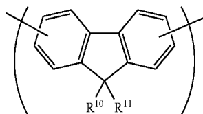
[Chemical Formula 15]
