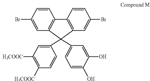
[Chemical Formula 82]
