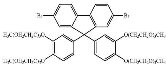
Compound G
