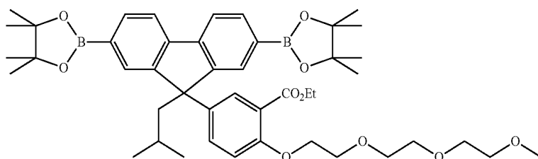
[Chemical Formula 77]
