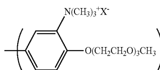
[Chemical Formula 18]
