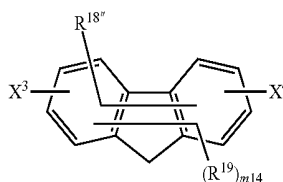
[Chemical Formula 51]
