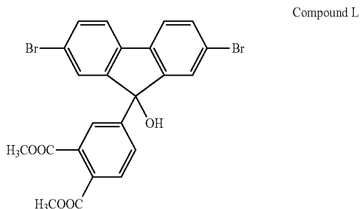
[Chemical Formula 81]
