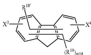
[Chemical Formula 48]
