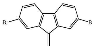
[Chemical Formula 54]
